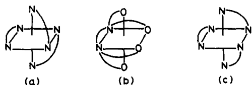
Fig. 10. Relationship between (a) \Delta\text{-(+)}_{589}\text{[Co(en)}_3\text{]}^{3+} , (b) \Delta\text{-(+)}_{546}\text{[Co(edta)]}^- and (c) \Delta\text{(-)}_{589}\text{[Co(en)}_3\text{]}^{3+} complex. (Reproduced with permission from ref. 75; copyright 1963 CSIRO, Australia.)
