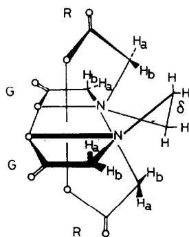
Fig. 1. The structure of \Lambda(\delta)-(-)_{546}-[\text{Co}(\text{edta})]^- complex.
