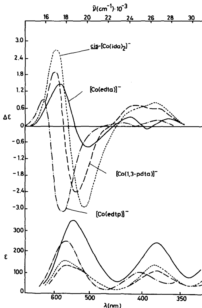
Fig. 13. CD and absorption spectra for \Lambda -(-) 46 -[Co(edta)] - and corresponding isomers of [Co(1,3-pdta)] - , cis -[Co(ida) 2 ] - and [Co(edtp)] - . (Reproduced with permission from ref. 83; copyright 1969 American Chemical Society.)
