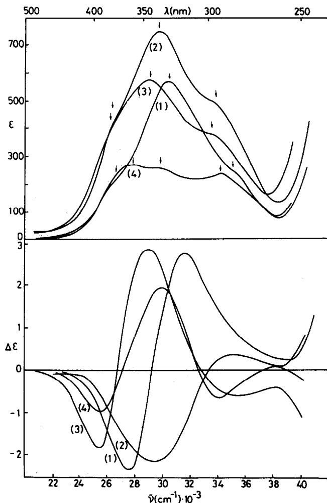
Fig. 14. CD and absorption spectra for [\text{Rh}(\text{edta-type})]^- complexes: (1) \text{trans}(\text{O}_5)\text{-}\Lambda\text{-(+)}_{\text{D}}\text{-}[\text{Rh}(\text{SS-edds})]^- ; (2) \text{trans}(\text{O}_5)\text{-}\Lambda\text{-(-)}_{\text{D}}\text{-}[\text{Rh}(\text{eddda})]^- ; (3) \text{trans}(\text{O}_5\text{O}_6)\text{-}\Lambda\text{-(-)}_{\text{D}}\text{-}[\text{Rh}(\text{eddda})]^- and (4) \Lambda\text{-(-)}_{\text{D}}\text{-}[\text{Rh}(1,3\text{-pdta})]^- .
