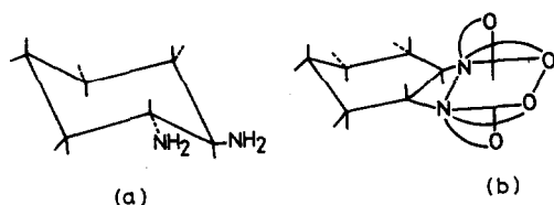
Fig. 7. The structure of (a) RR-trans -1,2-cyclohexanediamine, and (b) coordinated RR-trans -1,2-cyclohexanediaminetetraacetate in \Delta\text{-}(+)\text{_{546}}[\text{Co}(\text{RR-cdta})]^- complex.
