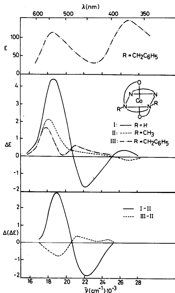
Fig. 23. CD spectra of the (+)- s-cis isomers of [\text{Co}(\text{edda})(\text{en})]^+ (I), [\text{Co}(\text{dmedda})(\text{en})]^+ (II), and [\text{Co}(\text{dbedda})(\text{en})]^+ (III) having \Delta absolute configuration (top) and difference curves: I–II and III–II (bottom).
