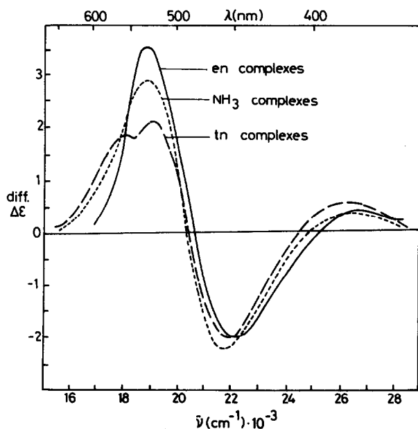
Fig. 21. Difference curves: \Delta\epsilon[\text{Co}(\text{edda})(L)]^+ - \Delta\epsilon[\text{Co}(\text{deedda})(L)]^+ ( L = tn, en and (\text{NH}_3)_2 ).
