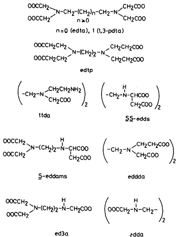
Fig. 5. The structure of the basic ligands. Optically active centers at the coordinated nitrogen donor atoms (ttda, \underline{\text{S}}\underline{\text{S}} -edds, \underline{\text{S}} -eddams, eddda, ed3a and edda ligands).
