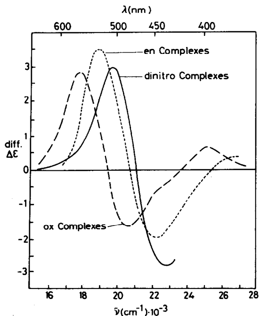
Fig. 22. Difference curves: \Delta\epsilon[Co(edda)(L)] - \Delta\epsilon[Co(dedda)(L)] ( L = ox, en and (NO_2)_2 ). (Reproduced with permission of ACS from ref. 179.)
