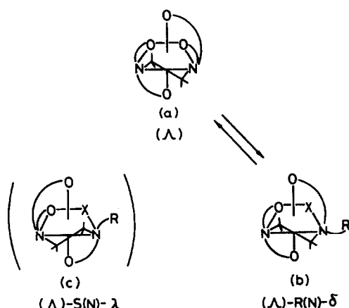
Fig. 17. Configuration relationship between \Lambda-( - )_{546}-[Co(edta)]^- and cis -eq ed3a-type complexes ( \Lambda configuration).
