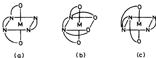
Fig. 20. Configurational comparison between: (a) \Lambda -(+)- s-cis -[Co(edda)(en)] + ; (b) \Delta -(+) 546 -[Co(edta)] - ; and (c) \Delta -(-)- s-cis -[Co(edda)(en)] + .
