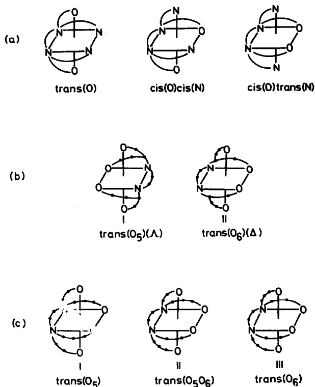
Fig. 2. Possible geometrical isomers of hexadentate complexes including various edta-type ligands: (a) ttda; (b) SS-edds; and (c) eddda.
