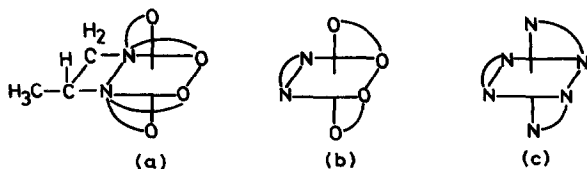
Fig. 9. Comparison between (a) \Delta-(+)_546^- [\text{Co}(\text{R-pdta})]^- , (b) \Delta-(+)_546^- [\text{Co}(\text{en})(\text{ox})_2]^- and (c) \Delta-(-)_589^- [\text{Co}(\text{en})_3]^{3+} (assigned the same L configuration [75]).
