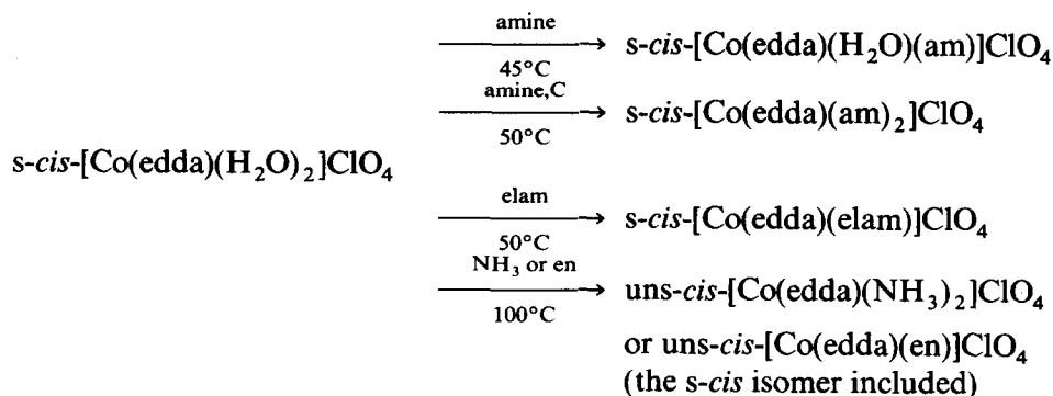
Scheme II. Preparation of [\text{Co(edda)}(\text{amine})]^+ complexes [168b].
